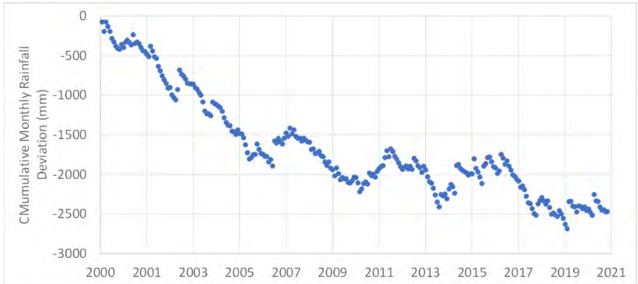
FIGURE 4-5: CUMULATIVE DEVIATION FROM MEAN MONTHLY RAINFALL AT CONCORD GOLF CLUB (BUREAU OF METEOROLOGY STATION 66013)
