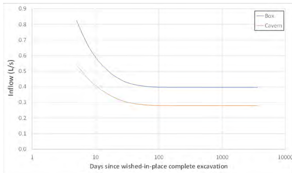
FIGURE 7-1: PREDICTED GROUNDWATER INFLOW RATES
