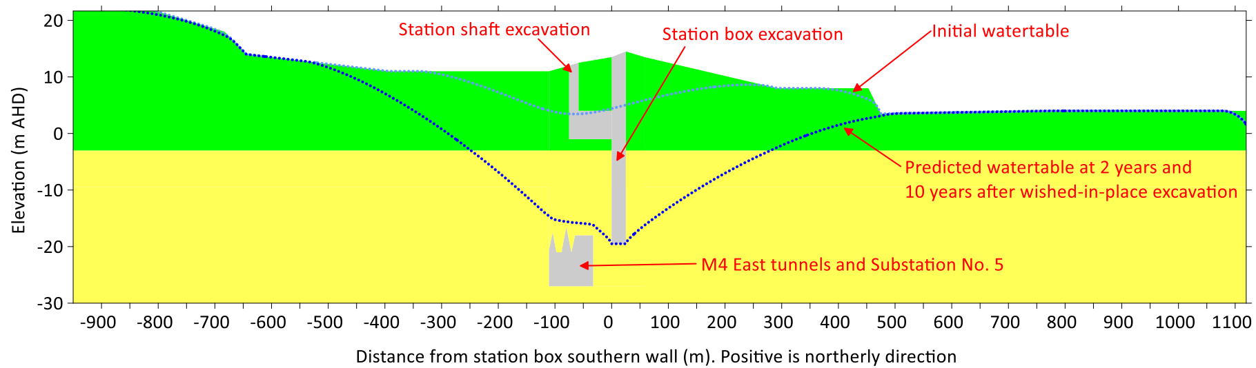
FIGURE 7-2: INTERPRETED PRE-CTP-WORKS EXCAVATION (INITIAL) WATERTABLE AND PREDICTED WATERTABLE AFTER (2 AND 10 YEARS SINCE) EXCAVATION, WITH SCENARIO IN WHICH DRAWDOWN AT M4 EAST INFRASTRUCTURE REACHED STEADY STATE PRIOR TO 2022
