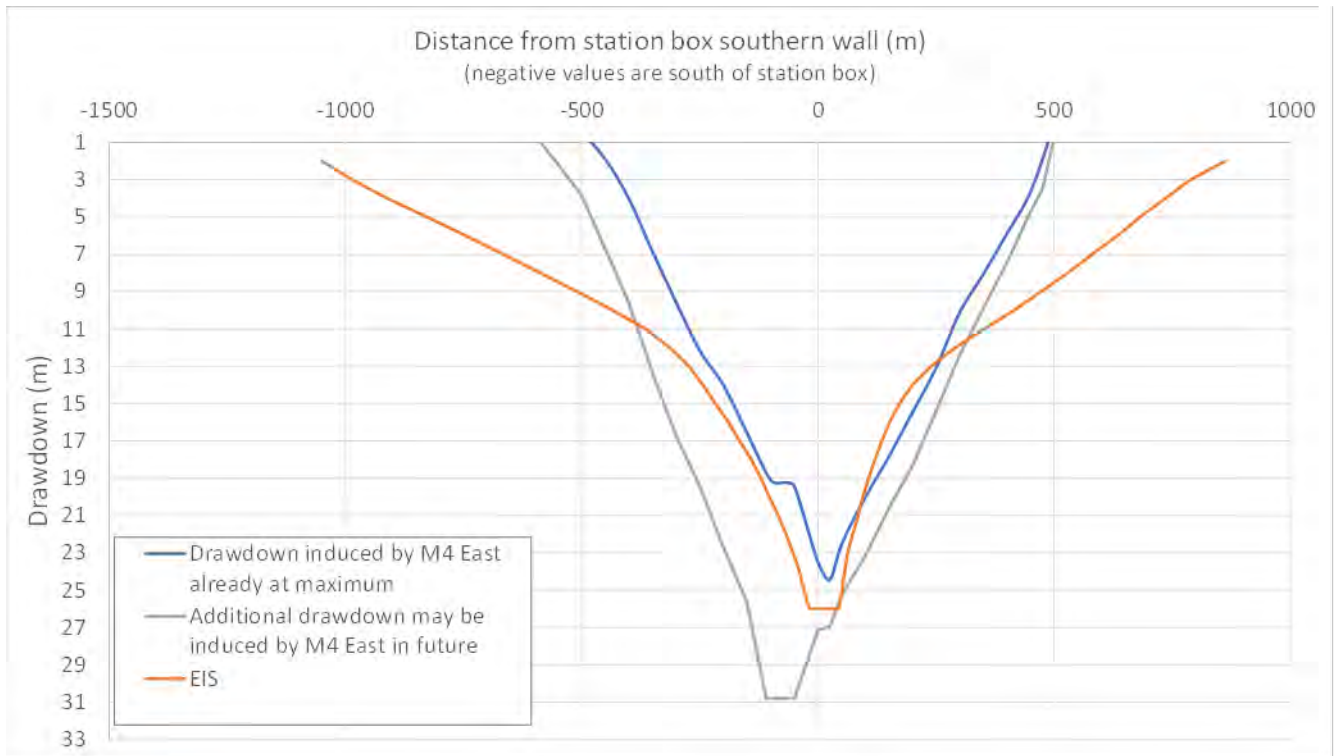
FIGURE 7-4: PREDICTED DRAWDOWN OF THE WATERTABLE AND DRAWDOWN PREDICTED IN THE EIS
