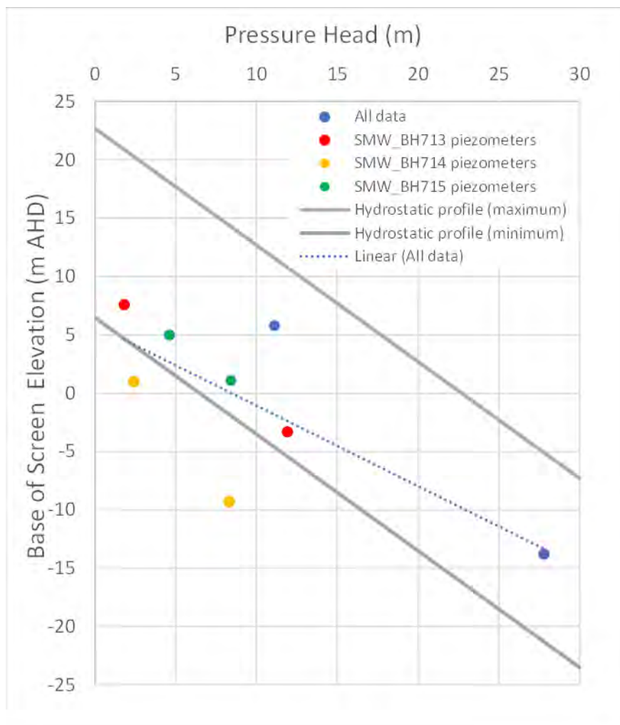
FIGURE 4-4: GROUNDWATER PRESSURE HEAD IN PIEZOMETERS AT BURWOOD NORTH STATION
