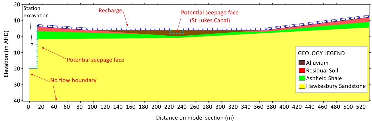
FIGURE 8 BURWOOD NORTH STATION – PALAEOCHANNEL MODEL CONDITIONS
