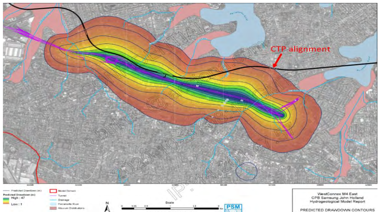
FIGURE 4-7: MODELLED GROUNDWATER DRAWDOWN FROM M4 EAST TUNNEL (FIGURE FROM CSJH, 2016)
