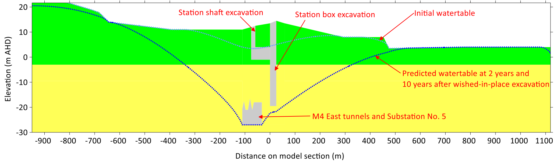
FIGURE 6 INTERPRETED PRE-CTP-WORKS EXCAVATION (INITIAL) WATERTABLE AND PREDICTED WATERTABLE AFTER (2 AND 10 YEARS SINCE) EXCAVATION, WITH SCENARIO IN WHICH DRAWDOWN AT M4 EAST INFRASTRUCTURE IS ONGOING IN 2022
