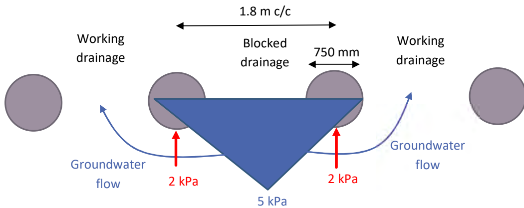
FIGURE 10: PRESSURE PROFILE DIAGRAM (IN PLAN VIEW)
