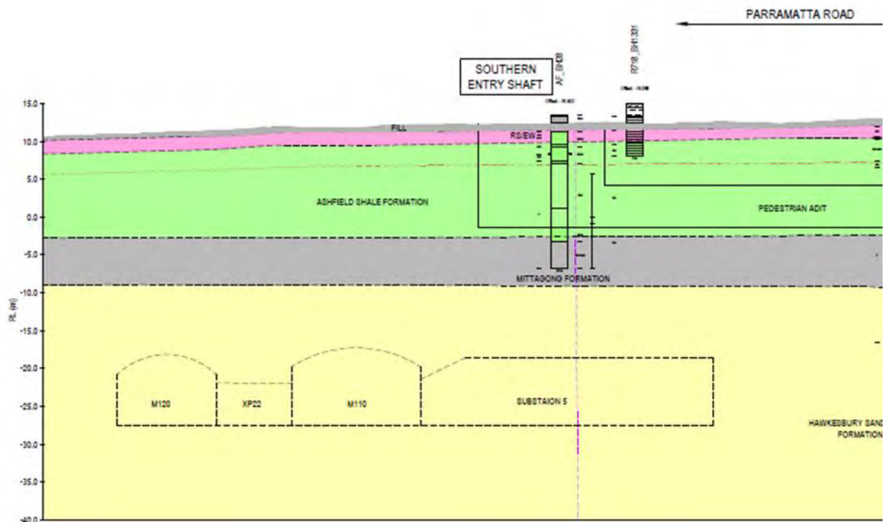
FIGURE 4-8: APPROXIMATE DEPTH OF BURWOOD NORTH STATION SHAFT AND M4 EAST TUNNELS AND SUBSTATION NO. 5
