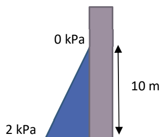
FIGURE 11: PRESSURE PROFILE TO ADOPT IN DESIGN OF SOIL RETAINING WALLS FOR EXCEPTIONAL LOAD CONDITION (GROUNDWATER) REPRESENTING BLOCKED DRAINAGE
