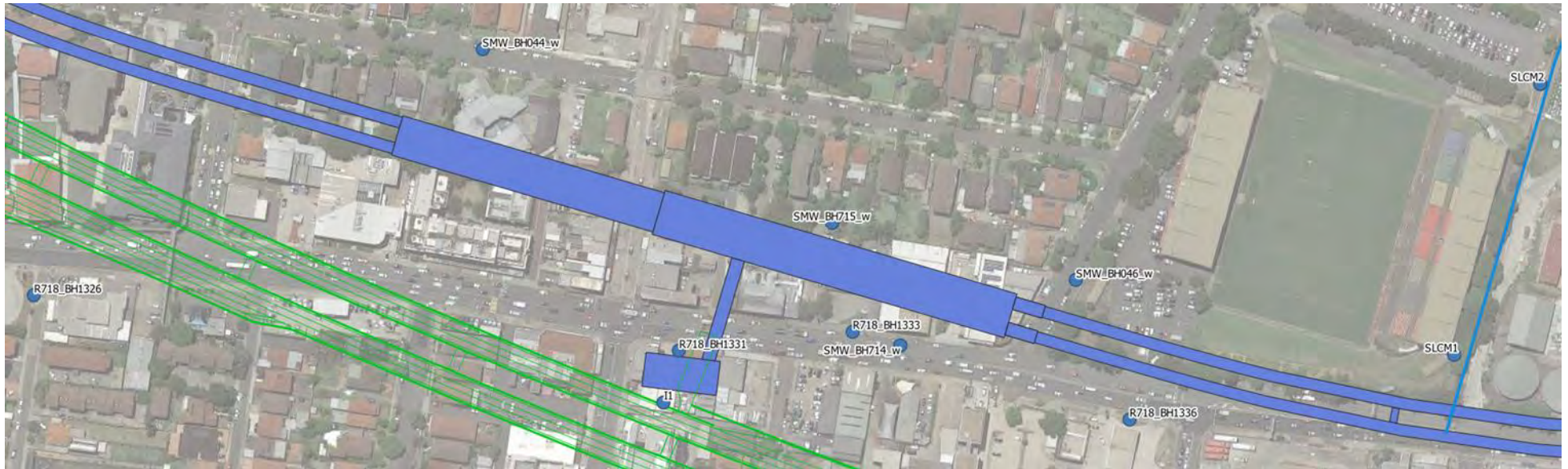
FIGURE 9-1: CONSTRUCTION PHASE GROUNDWATER LEVEL MONITORING LOCATIONS
