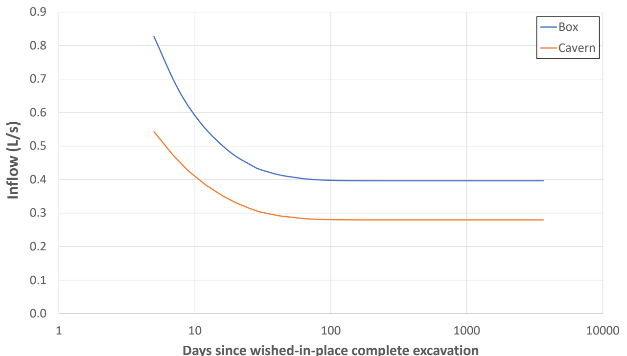
FIGURE 4 PREDICTED GROUNDWATER INFLOW RATES
