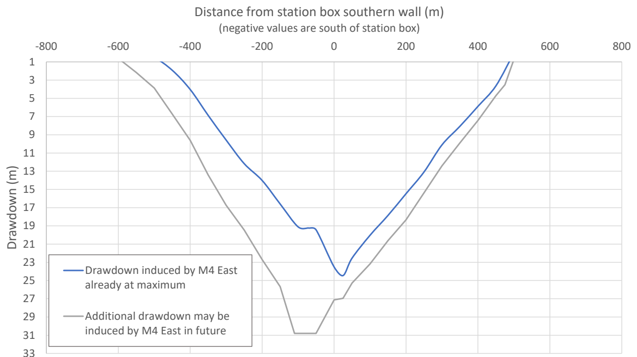
FIGURE 7 PREDICTED DRAWDOWN OF THE WATERTABLE
