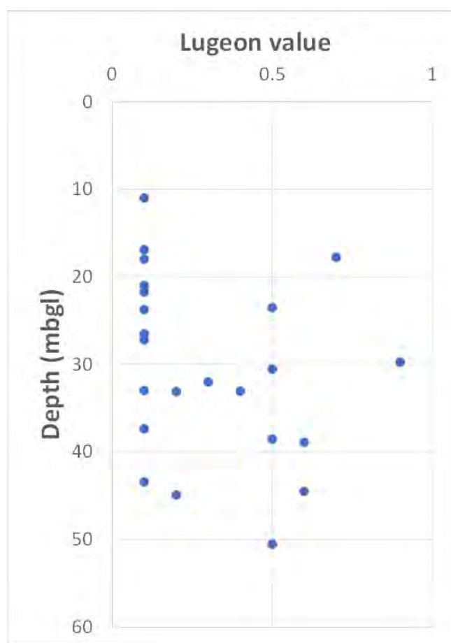
FIGURE 4-10: LUGEON VALUES WITH DEPTH BELOW GROUND SURFACE
