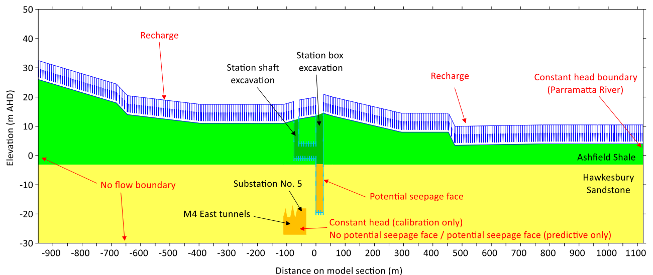
FIGURE 2 BURWOOD NORTH STATION MODEL CONDITIONS
