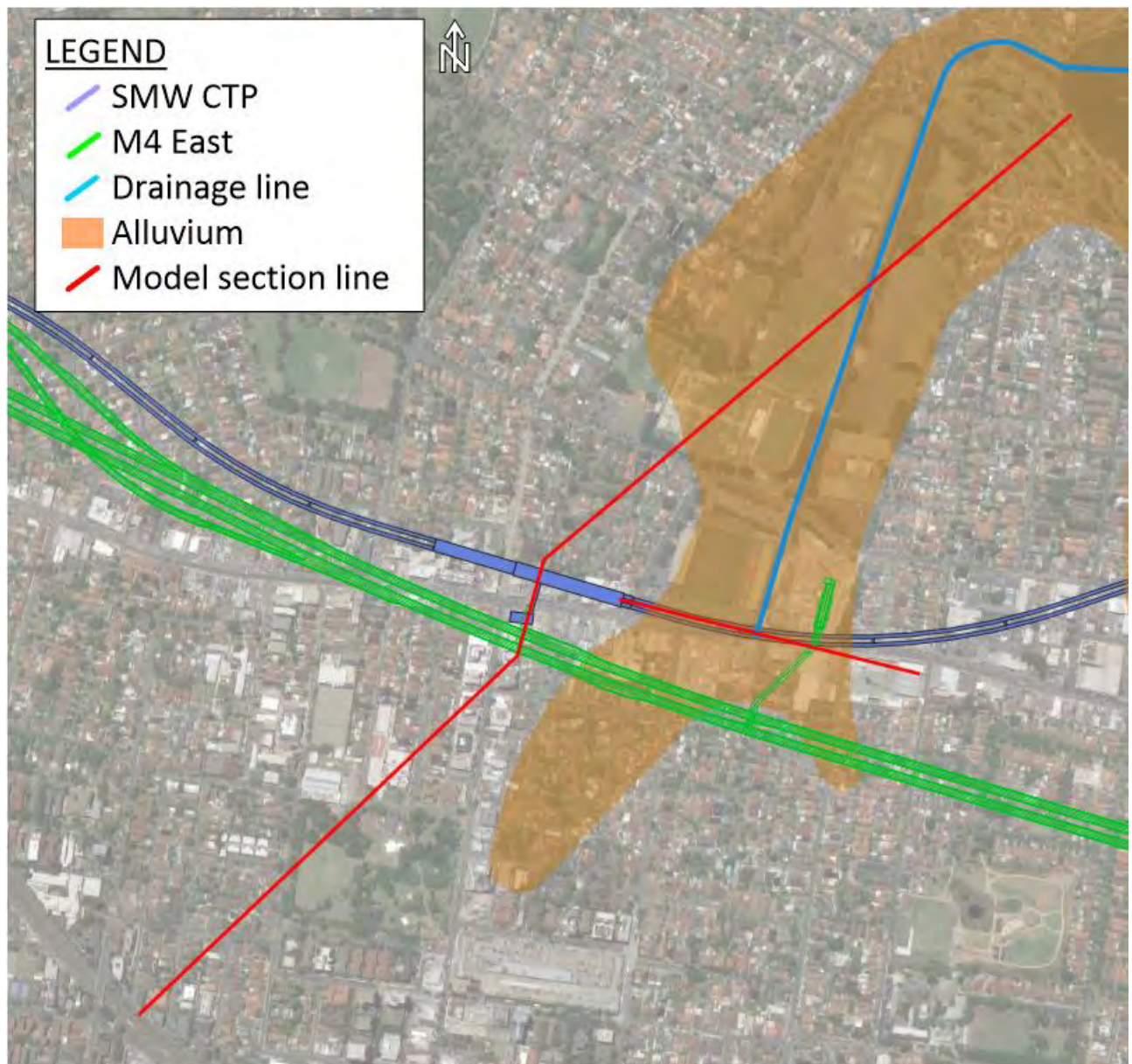
FIGURE 1 BURWOOD NORTH STATION – STATION MODEL AND PALAEOCHANNEL MODEL CROSS SECTION LOCATIONS
