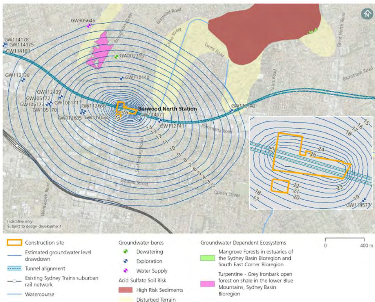
FIGURE 8-1: GROUNDWATER RECEPTORS NEAR BURWOOD NORTH STATION AND PREDICTED GROUNDWATER LEVEL DRAWDOWN FROM THE EIS (JACOBS, 2020)
