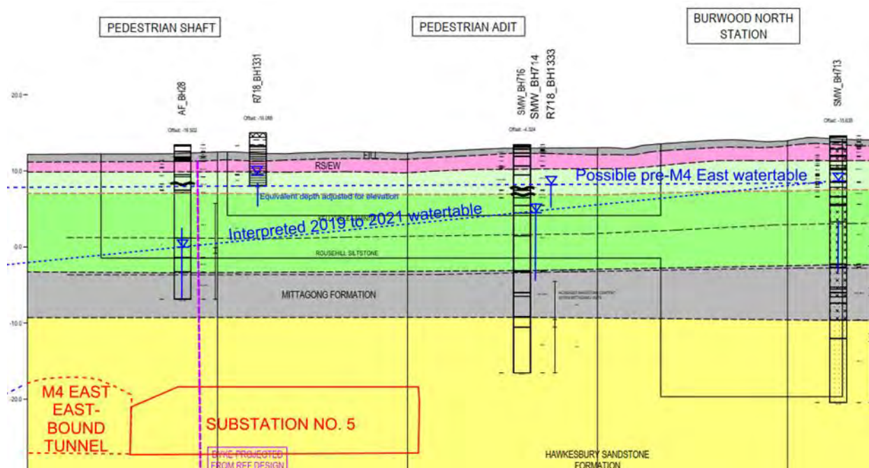
FIGURE 4-9: INTERPRETED GROUNDWATER LEVELS BETWEEN BURWOOD NORTH STATION AND M4 EAST TUNNELS/SUBSTATION NO. 5
