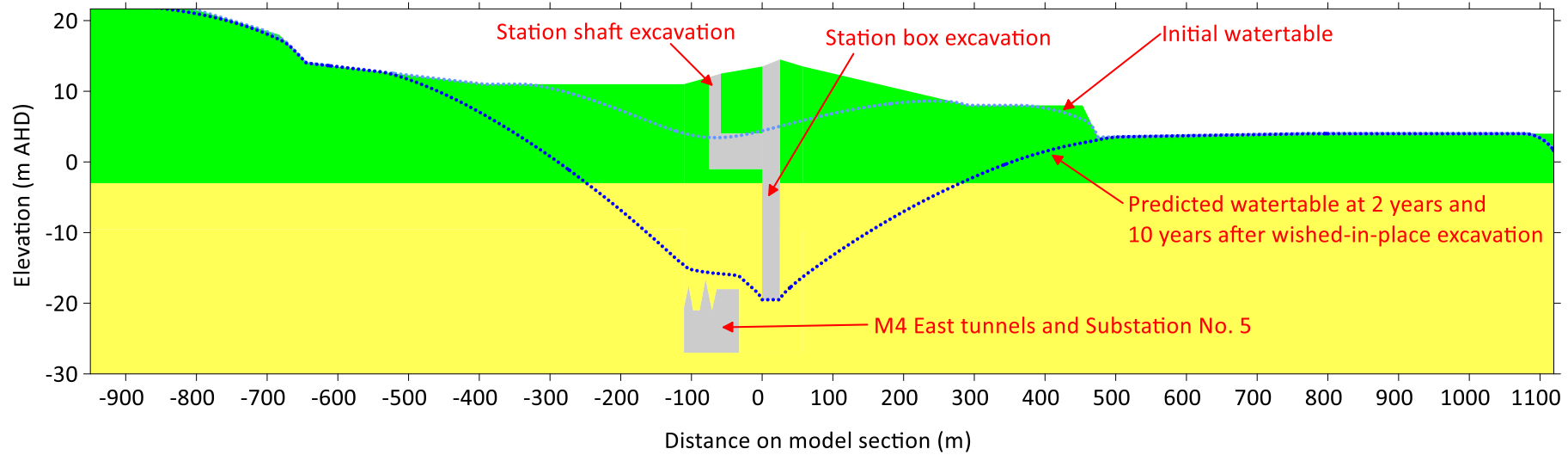
FIGURE 5 INTERPRETED PRE-CTP-WORKS EXCAVATION (INITIAL) WATERTABLE AND PREDICTED WATERTABLE AFTER (2 AND 10 YEARS SINCE) EXCAVATION, WITH SCENARIO IN WHICH DRAWDOWN AT M4 EAST INFRASTRUCTURE REACHED STEADY STATE PRIOR TO 2022
