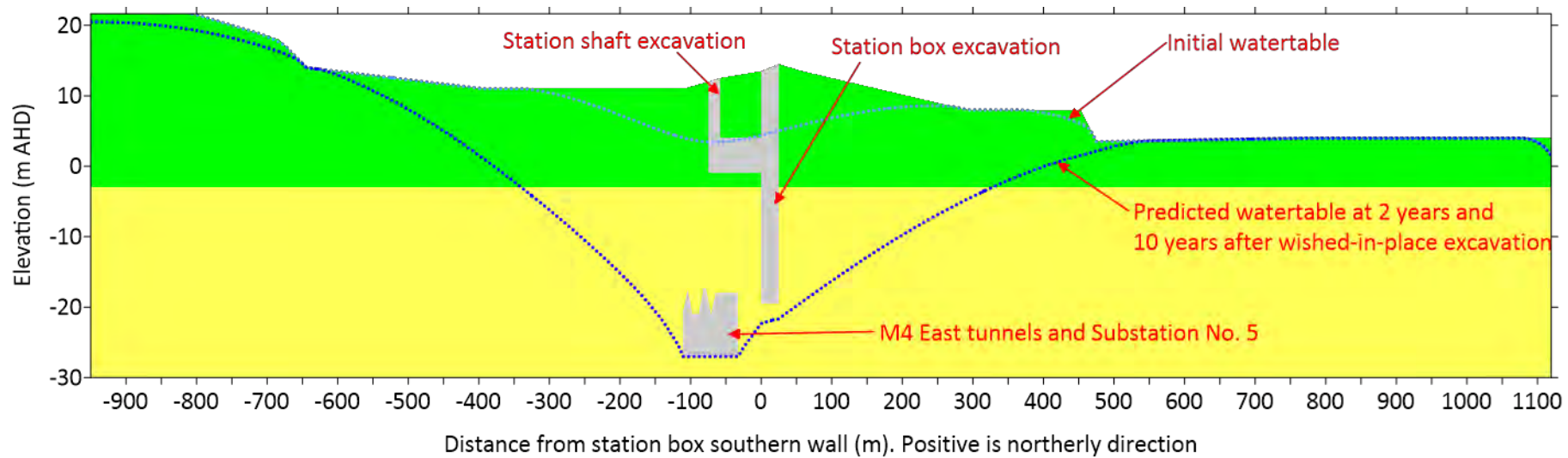
FIGURE 7-3: INTERPRETED PRE-CTP-WORKS EXCAVATION (INITIAL) WATERTABLE AND PREDICTED WATERTABLE AFTER (2 AND 10 YEARS SINCE) EXCAVATION, WITH SCENARIO IN WHICH DRAWDOWN AT M4 EAST INFRASTRUCTURE IS ONGOING IN 2022
