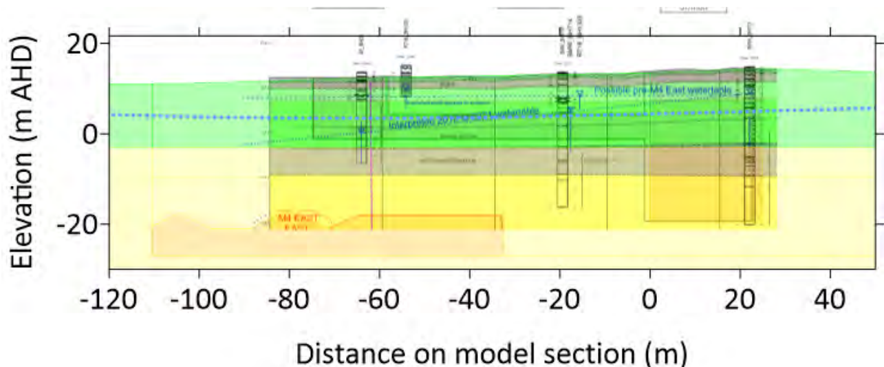
FIGURE 3 CALIBRATED WATERTABLE LEVEL (BLUE DASHED LINE)
